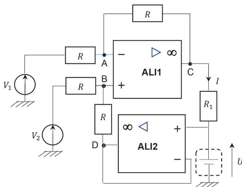
Figure 12 - Dispositif de charge
