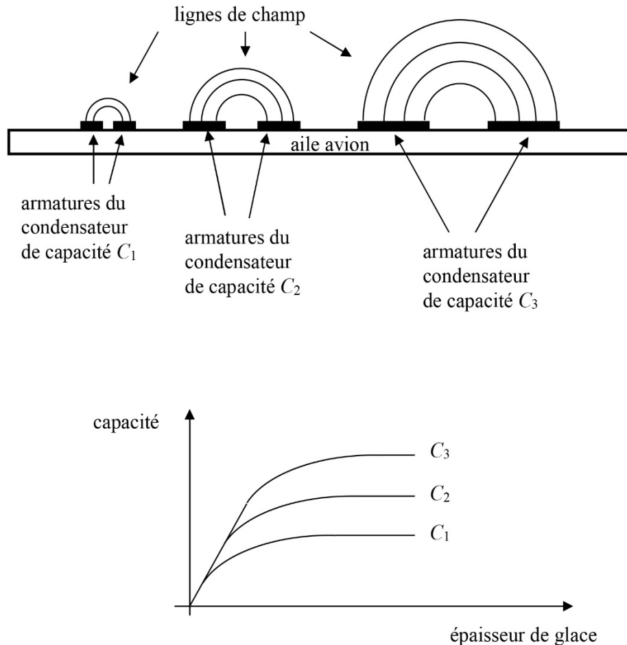
Figure 11 - Mesure capacitive
