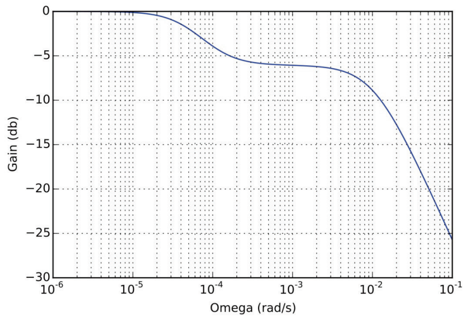
FIGURE 10 – Diagramme de Bode sans isolation
